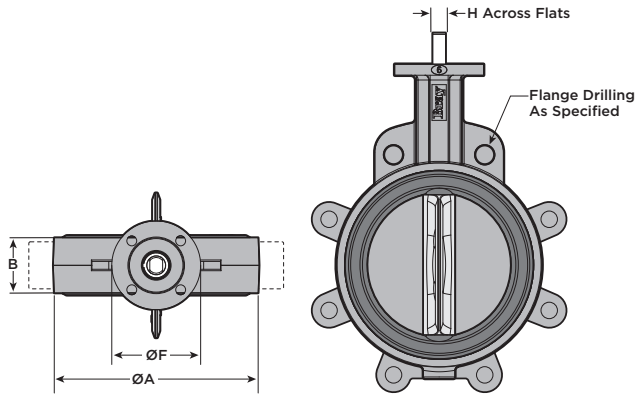
VALVE BODY DIMENSIONS in. (mm)
