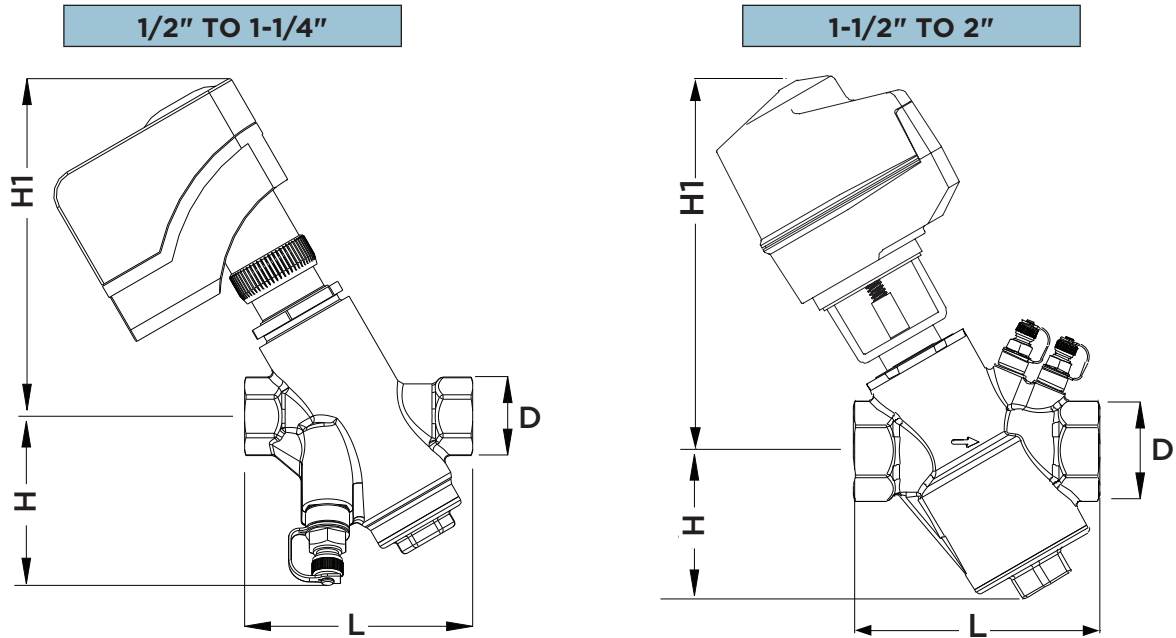
Simple Set - Technical Data and Dimensions
